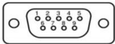
Connector Pinout
